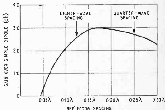
Fig. 3. Variation of gain of dipole and reflector over dipole alone with reflector spacing when the reflector length is adjusted for the optimum front-to-back ratio.
