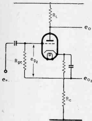
Normal cathode-follower phase-splitter.
