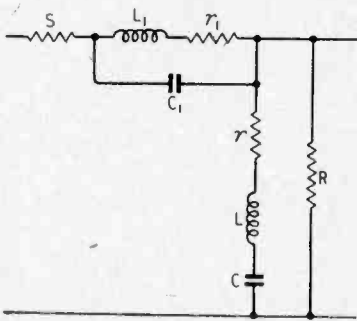
Fig. 3. Circuit with the addition of a rejector for the 3,000 c/s needle resonance.
