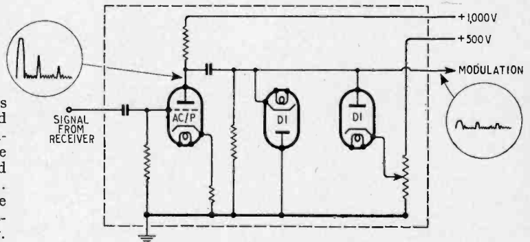
Fig. 2. Complete circuit diagram of radial time base.
