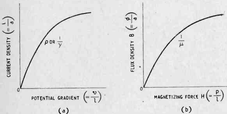
Fig. 5. When the non-linearity of a resistor is a peculiarity of the material of which it is made, it is more helpful to have a graph of the material, rather than of any particularly-sized piece of it, as would be shown in a Fig. 2b type of graph. This is done by altering the co-ordinate scales, as at a . The same argument applies to magnetic materials, which accounts for their graphs usually being plotted as at b (compare a ) instead of as Fig. 4b.
