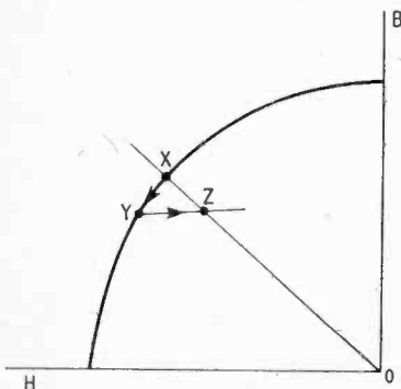
Fig. 9. If a magnetic circuit originally working at point X is demagnetized somewhat, say to Y; removing the demagnetizing influence causes it to return, not to X but to Z. To avoid the loss XZ taking place during service, magnets are previously brought by "aging" on to a flat curve like YZ.
