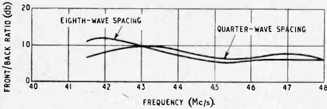
Fig. 6. Measured front-to-back ratios for \lambda/8 and \lambda/4 spaced reflectors.
