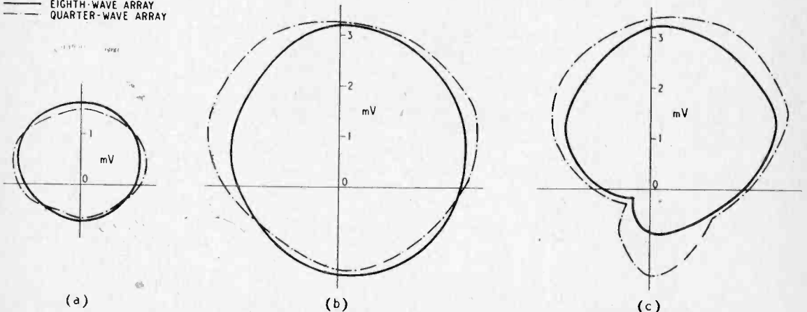
Fig. 7. Polar diagrams of \lambda/8 and \lambda/4 spaced reflector systems at 48 Mc/s (a), 45 Mc/s (b) and 41.5 Mc/s (c).
