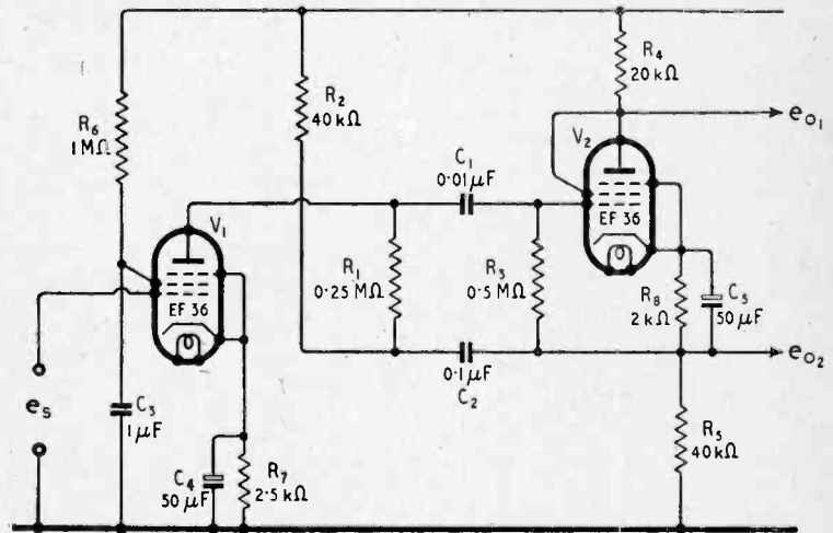
Fig. 4. The practical form of the high-gain phase-splitter and preceding stage.
