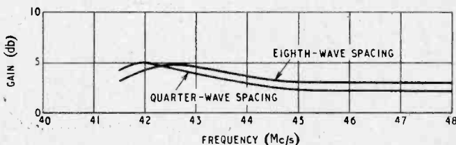
Fig. 5. Measured forward-gain curves of \lambda/8 and \lambda/4 spaced reflectors.
