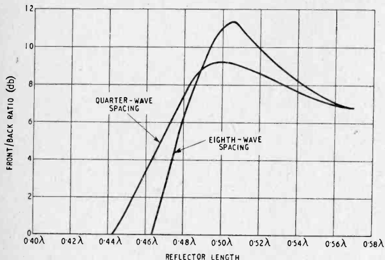
Fig. 4. The effect of the reflector length on the front-to-back ratio is shown here for reflector-aerial spacings of \lambda/8 and \lambda/4 .
