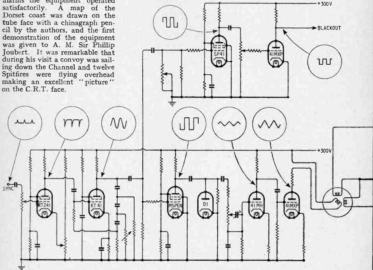
Fig. 2. Complete circuit diagram of radial time base.
