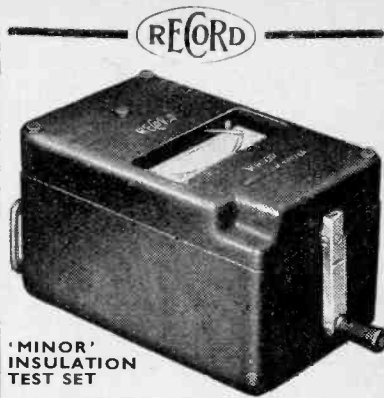
'MINOR' INSULATION TEST SET Compact and inexpensive without sacrificing accuracy and reliability. Weighs only 3lb. Height allows for full swing of generator handle. Ranges up to 20 megohms 500 volts.
