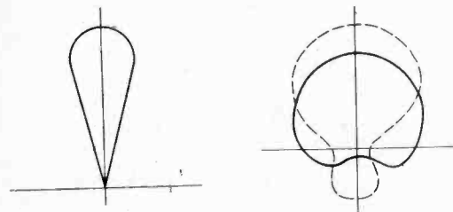
Fig. 1 (left). Ideal directional pattern obtainable only with multi-element array. Fig. 2 (right). Specimen patterns obtainable with single reflector.
