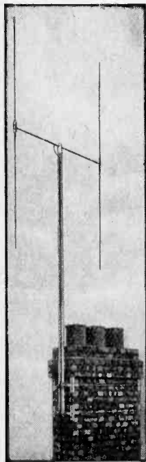
U.K. PATENT No. 526587. This Patent is concerned with the cap shaped mast head fixing (Fig. 3).
